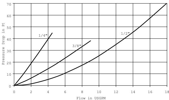
4000 Series (1/4", 3/8", 1/2") Test Fluid: Oil - 200 SUS
